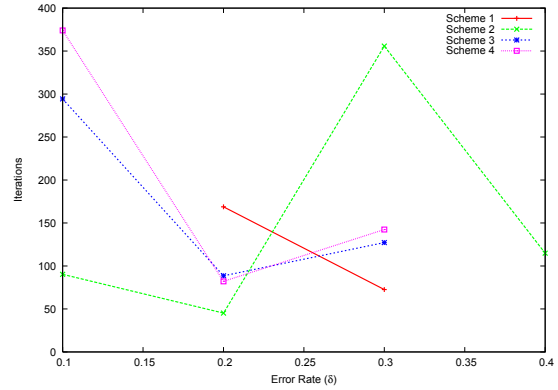
Figure 9: Sign Test results with Error Model 3.
