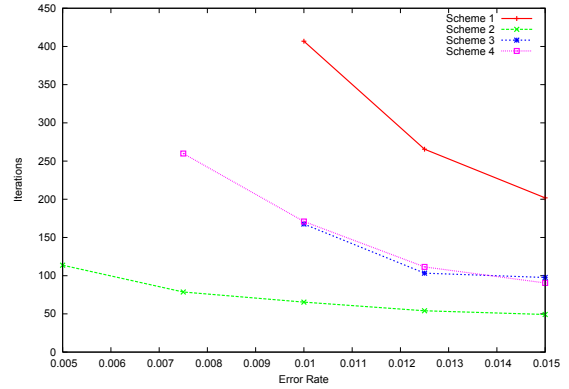
Figure 8: Sign Rank Test results for Error Model 2.
